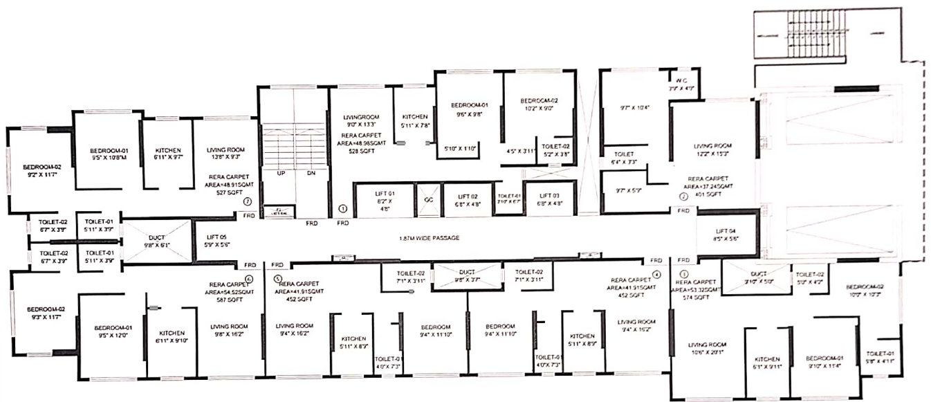
TYPICAL FLOOR PLAN 11TH - 13TH, 14TH, 16TH TO 19TH
