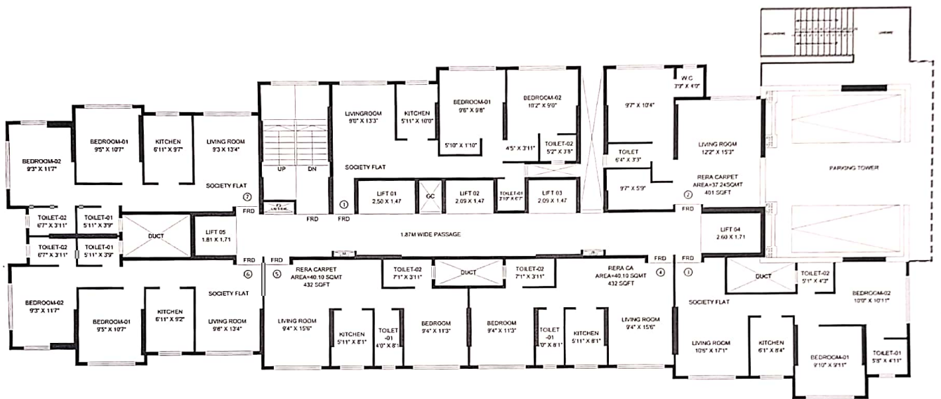
TYPICAL FLOOR PLAN 2ND TO 7TH - 9TH TO 10TH
