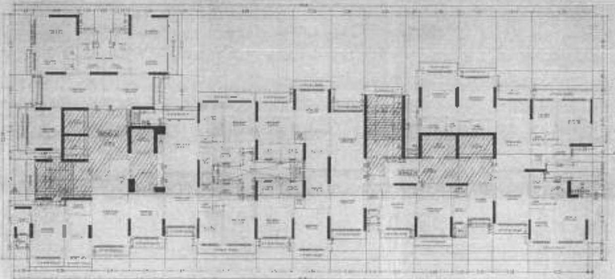
TYPICAL 1ST TO 18TH FLOOR PLAN
