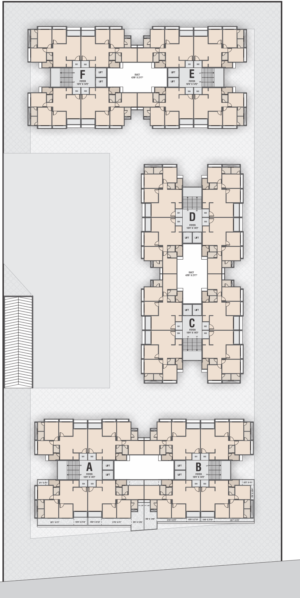
FIFTH_FLOOR PLAN
