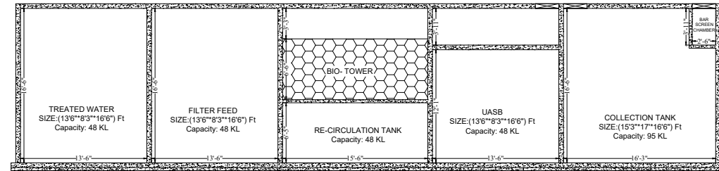
SECTION X-X
