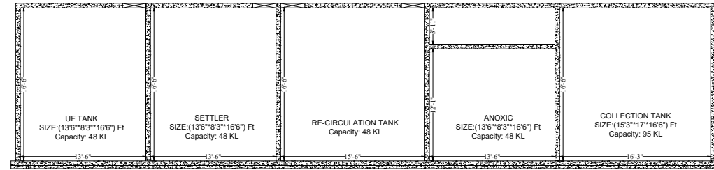
SECTION Y-Y
