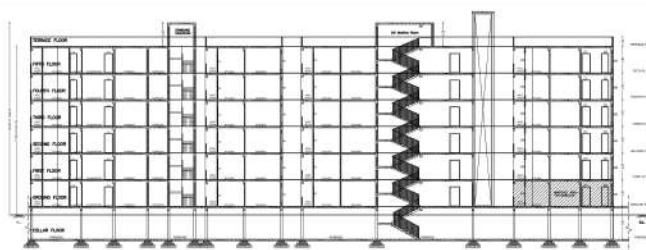
SECTION AT A-A (SCALE 1:200)
