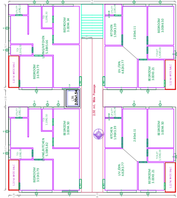
TYPICAL - 2, 3, 4& 5 FLOOR PLAN (SCALE=1:100)
