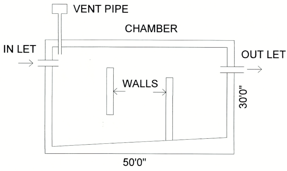
SECTION
