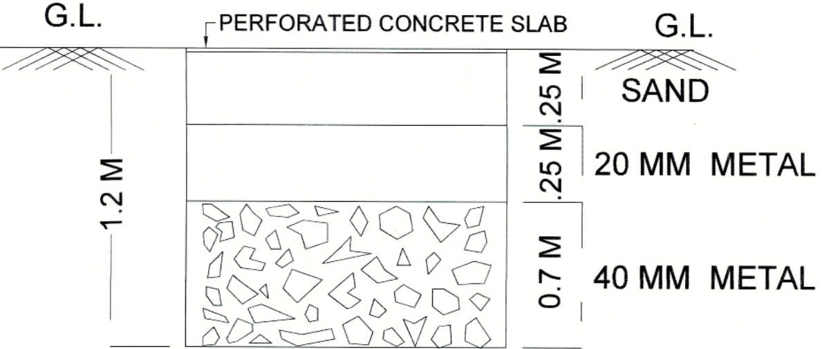
SECTION
