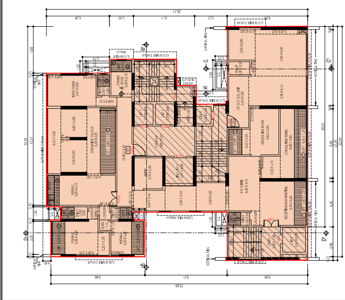
1ST FLOOR PLAN SCALE - 1:100
