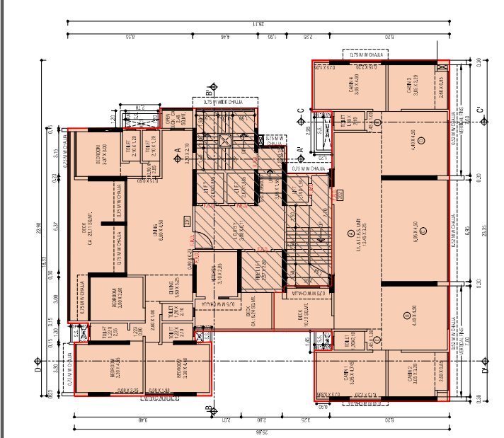
2ND FLOOR PLAN SCALE - 1:100
