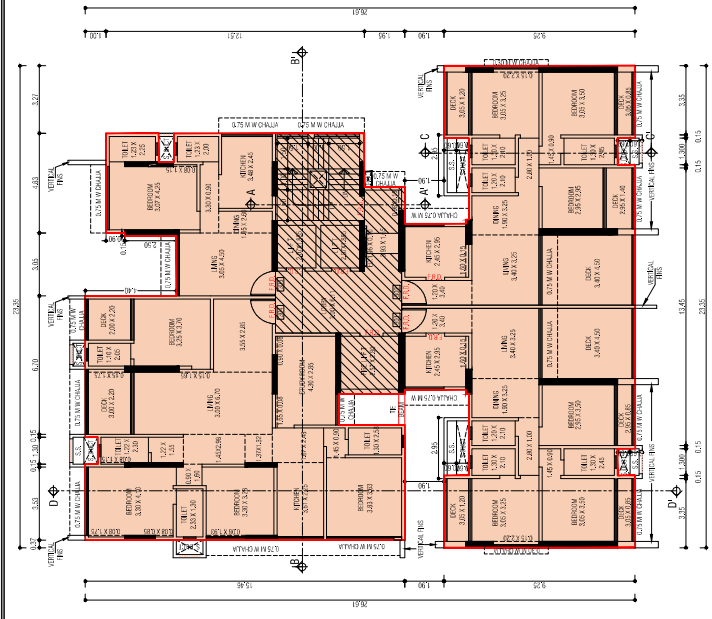
3RD FLOOR PLAN SCALE - 1:100
