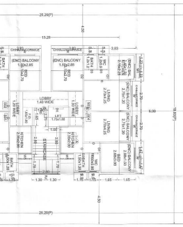
FIFTH FLOOR PLAN
