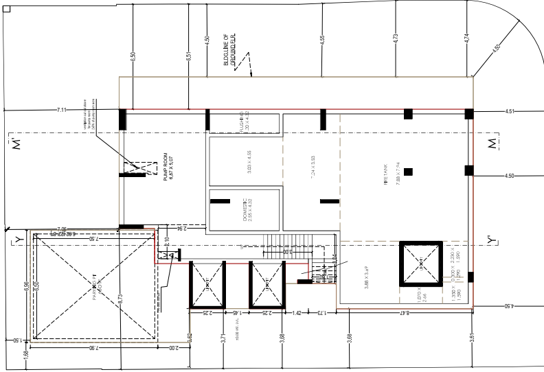
<--- C R O S S R O A D NO.1 ---> BASEMENT FLOOR PLAN
