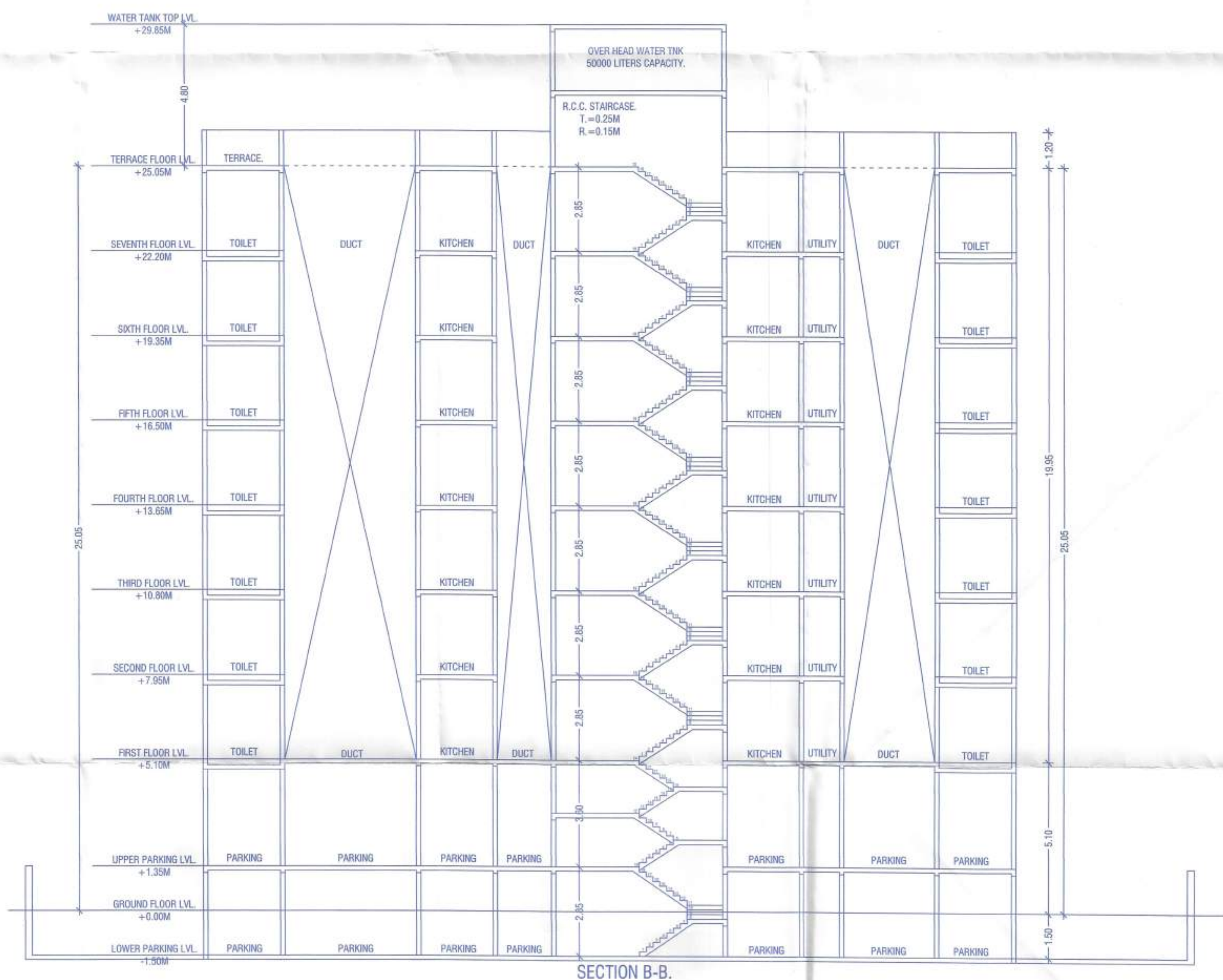
SECTION B-B.
