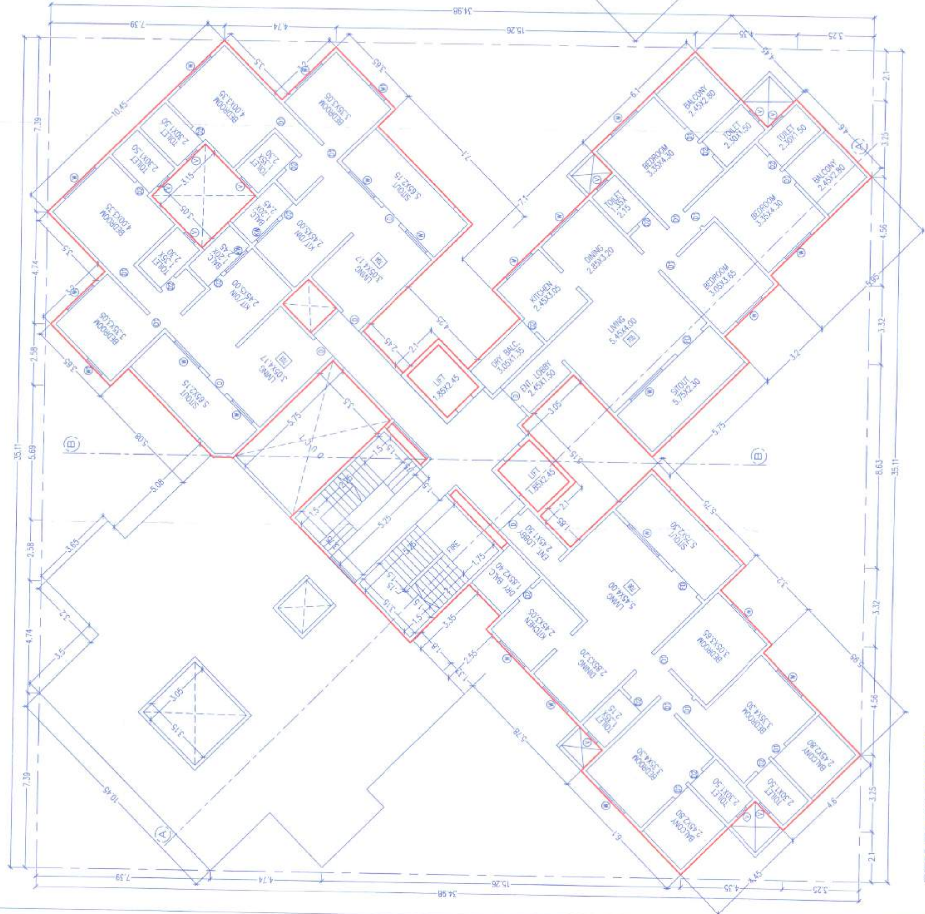
7TH FLOOR PLAN
