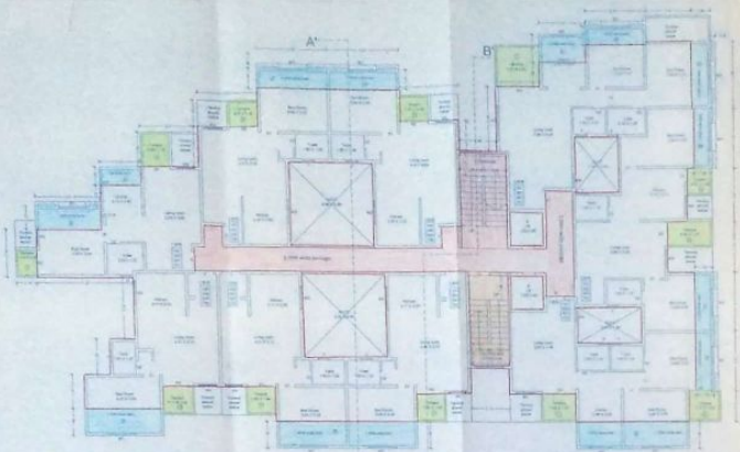
1st, 3rd, 5th, 7th FLOOR PLAN SCALE: 1:100
