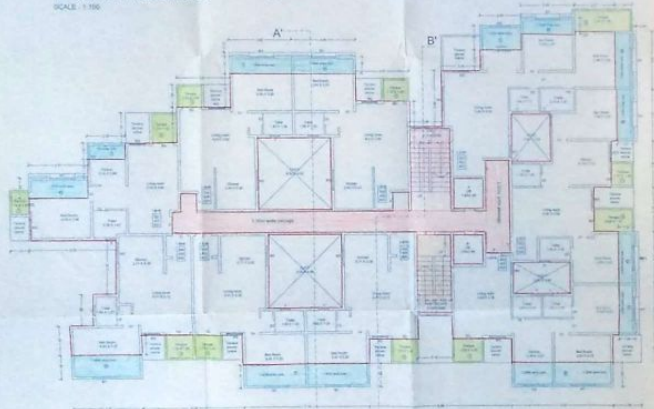
2nd, 4th & 6th FLOOR PLAN SCALE: 1:100
