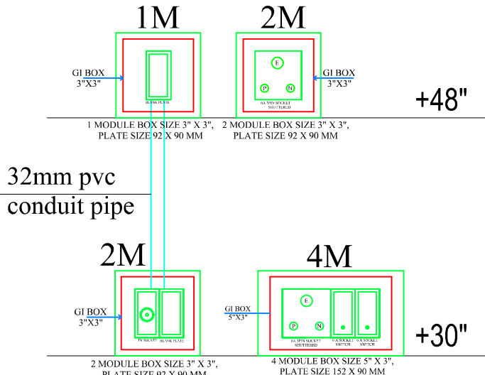
TYPICAL TV WALL ELEVATION PLAN
