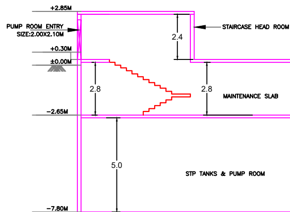
SECTION-B
