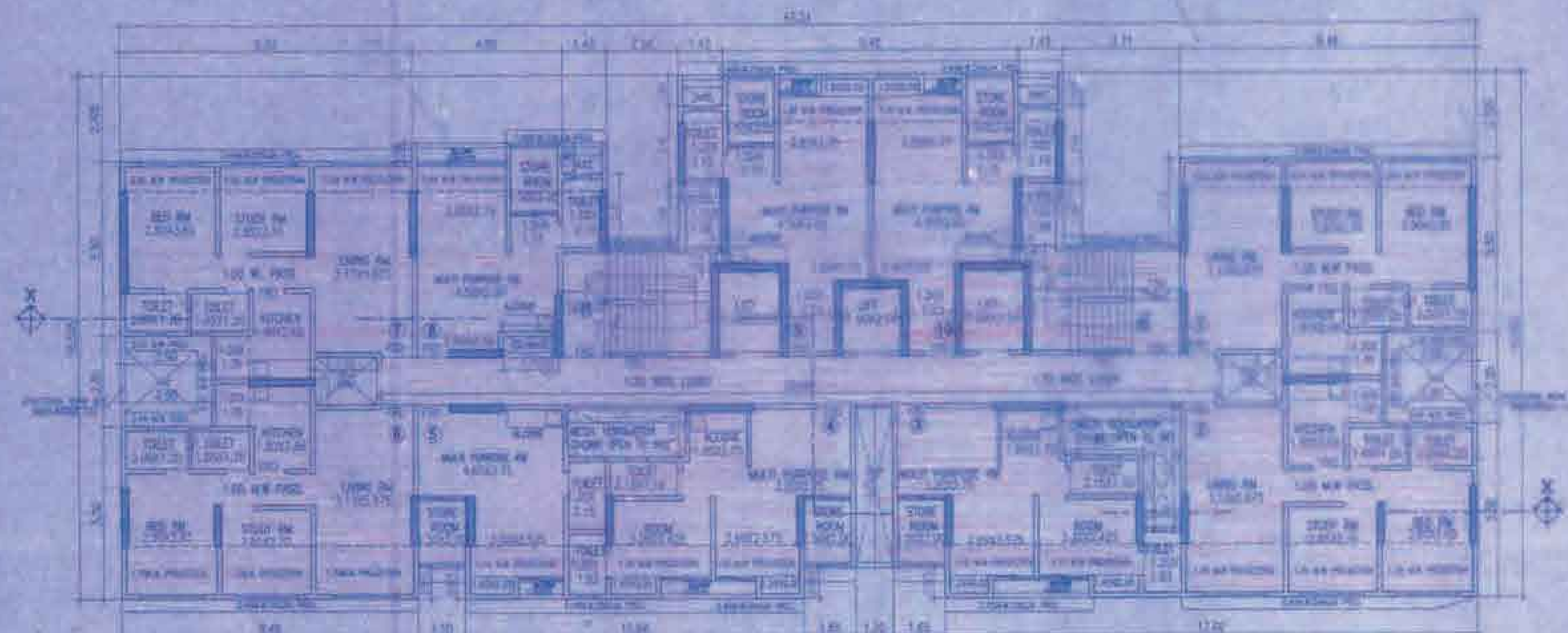
TYPICAL FLOOR PLAN 2ND TO 4TH FLOOR SCALE 1:100
