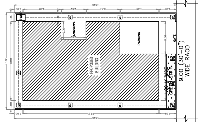
GROUND FLOOR PLAN (SCALE 1:100)
