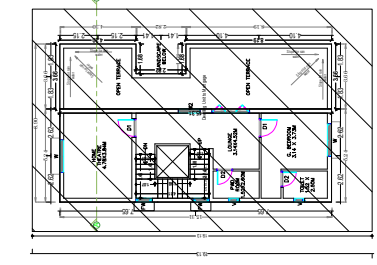
SECOND FLOOR PLAN (SCALE 1:100)
