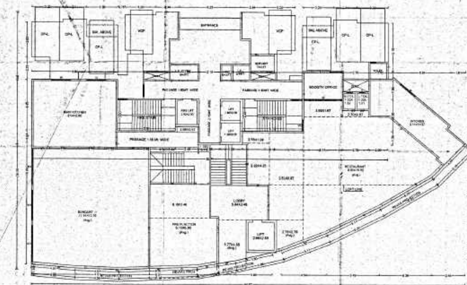
PODIUM FLOOR PLAN
