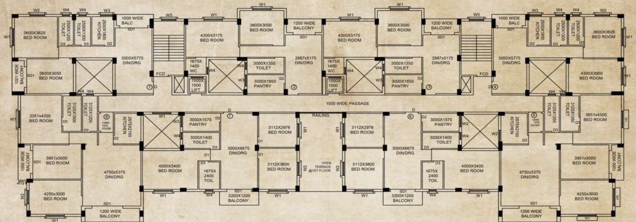
BLOCK-C 1ST TO 7TH FLOOR PLAN
