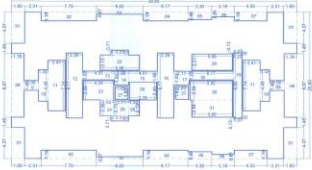
UPPER GROUND, 1ST, 2ND & 3RD FLOOR AREA KEY PLAN
