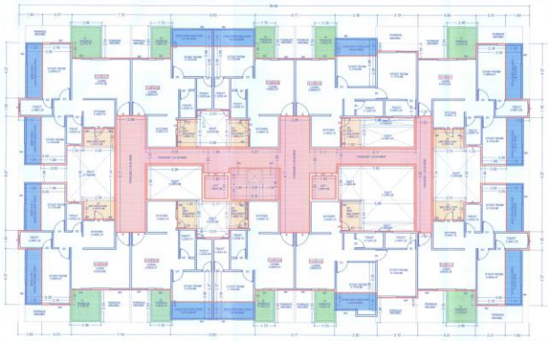
FIRST & THIRD FLOOR PLAN WING - C
