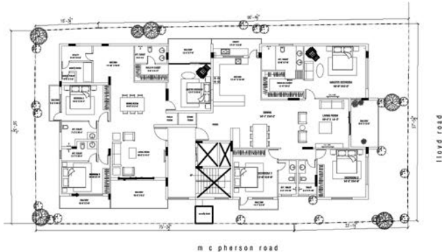
FIRST FLOOR PLAN PROPOSED RESIDENTIAL BUILDING FOR M. PRAGNATHI RAO, AT BANGALORE
