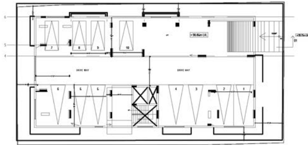
BASEMENT FLOOR PLAN PROPOSED RESIDENTIAL BUILDING FOR M. PRAGNATHI RAO, AT BANGALORE
