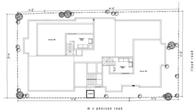
TERRACE FLOOR PLAN PROPOSED RESIDENTIAL BUILDING AT NO 12, LLOYD ROAD BANGALORE
