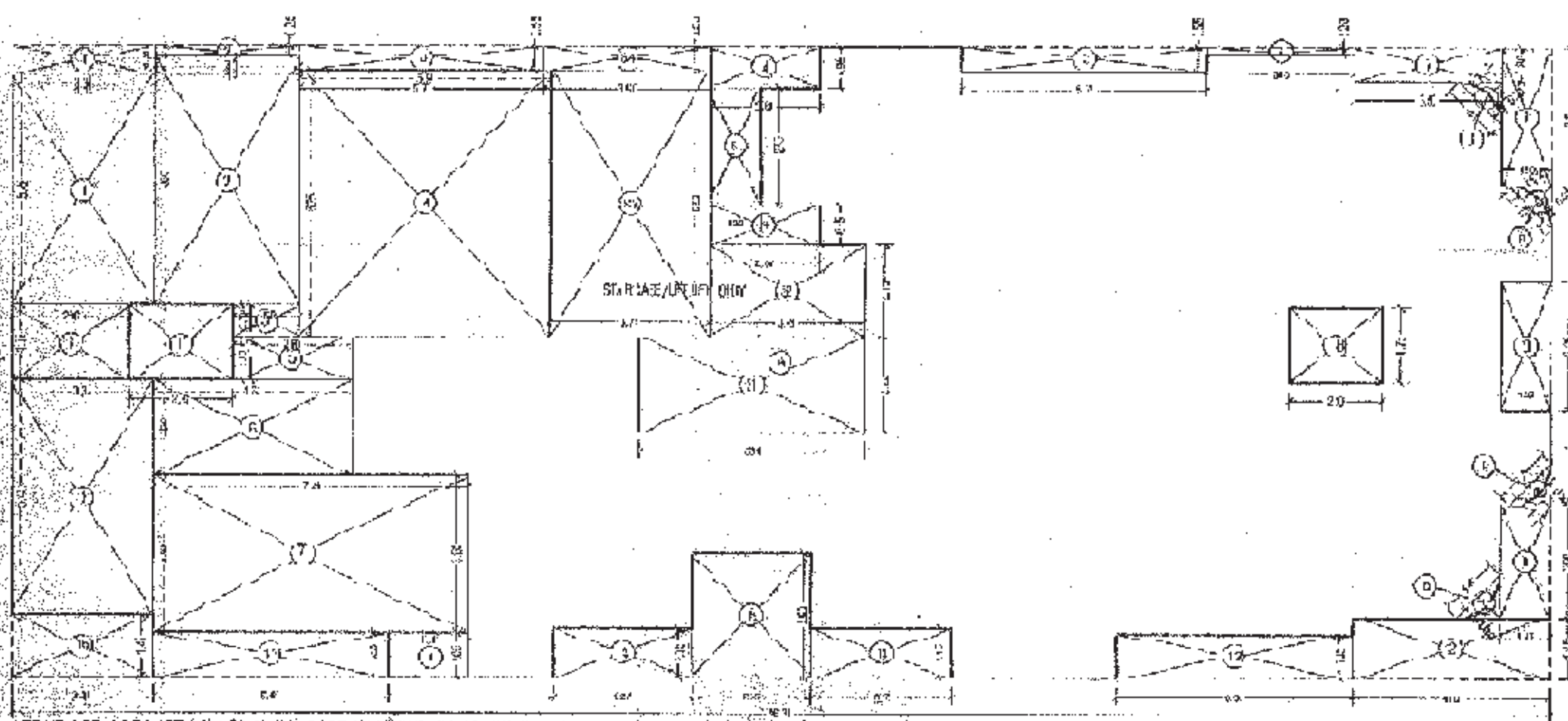
ARCHITECTURAL DRAWING OF 10TH FLOOR PLAN OF COMPOSITE BUILDING NO. 01 (SALEM - A)
