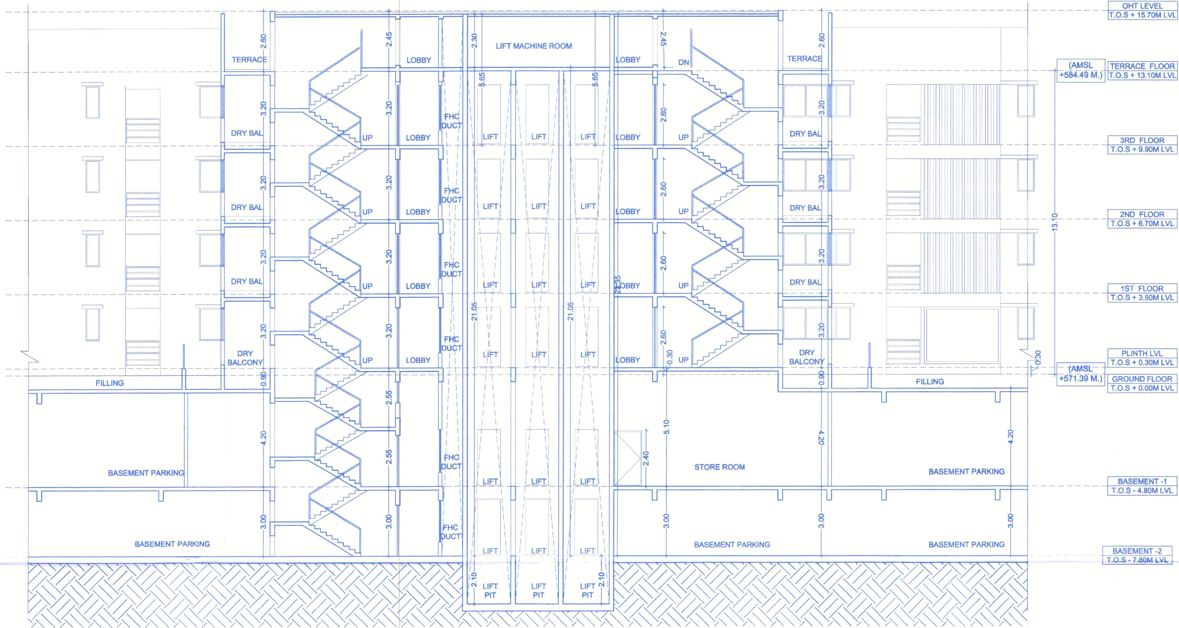
TOWER-1: SECTION AT - 1A (SCALE 1:100)
