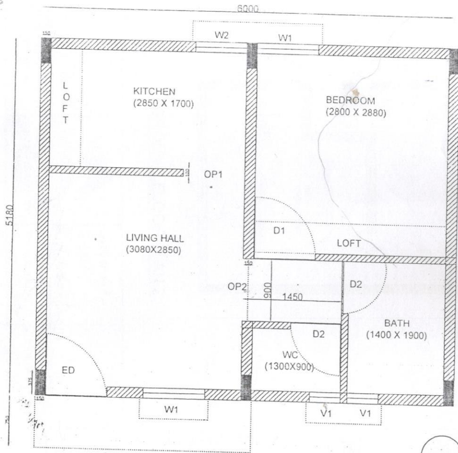
GROUND FLOOR PLAN 1
