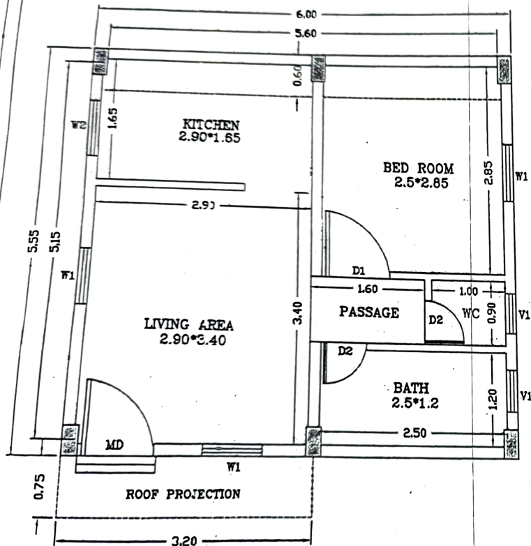
PLAN AT SILL LEVEL
