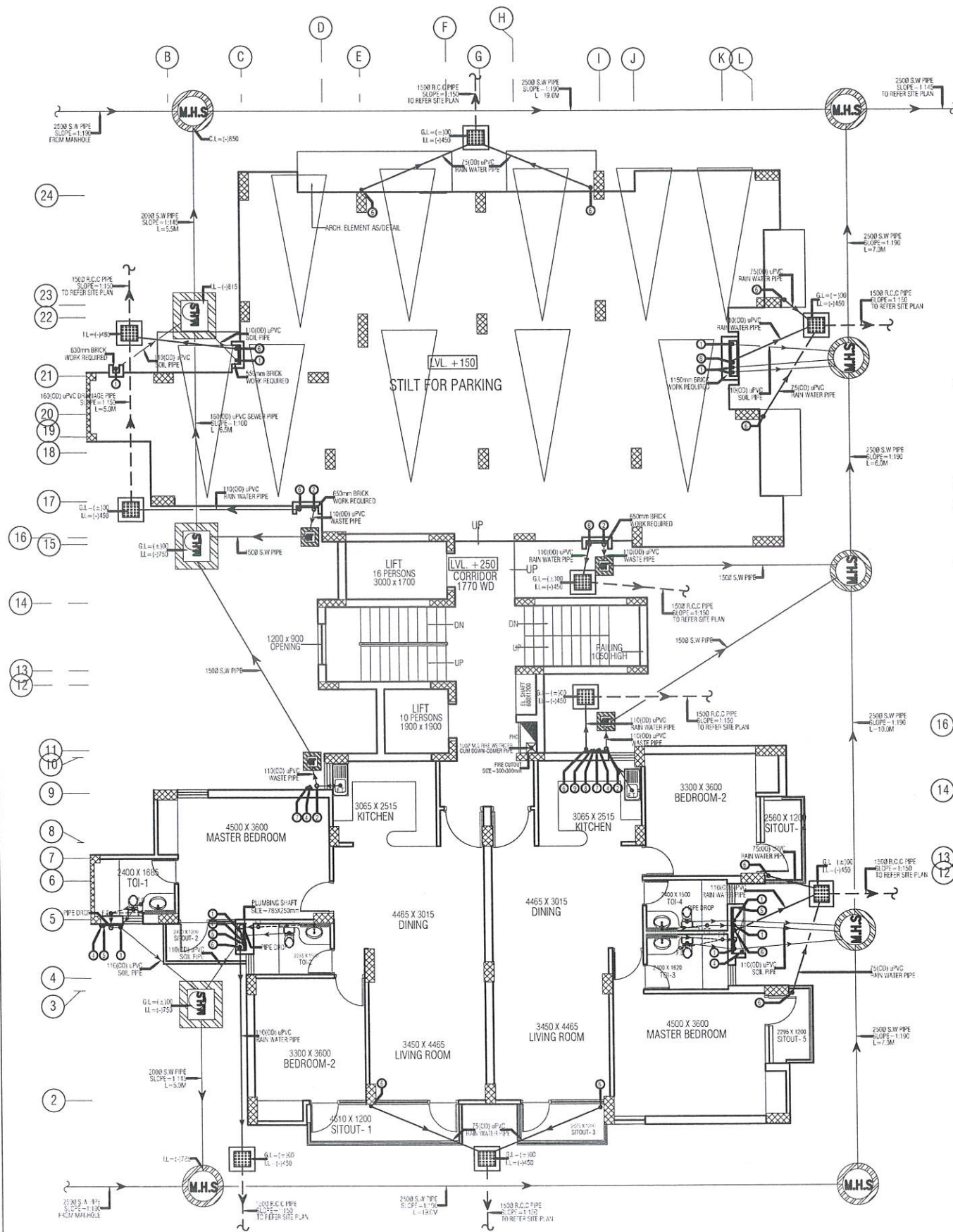
STILT PLAN
