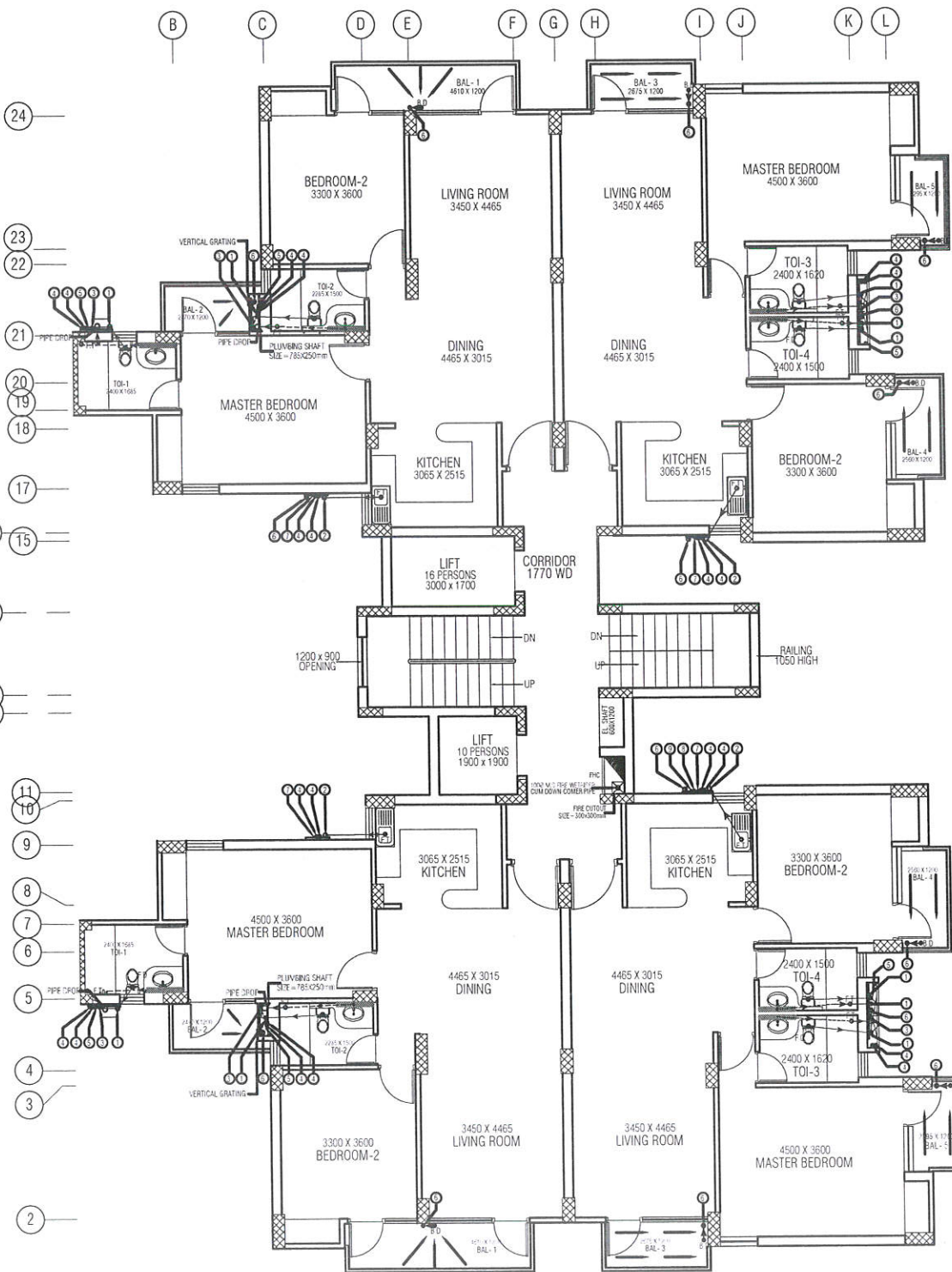
TYPICAL PLAN
