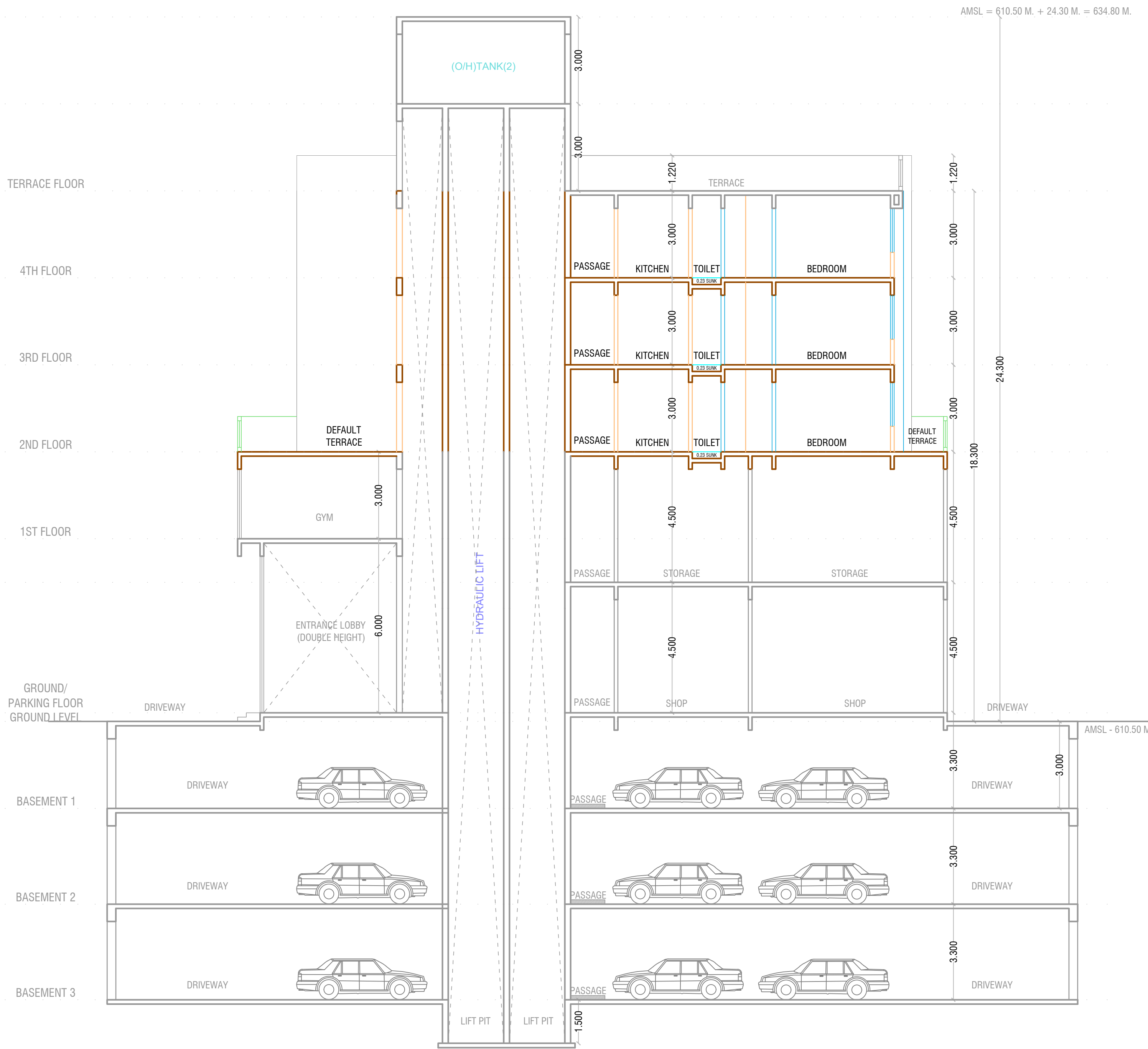
SECTION B
