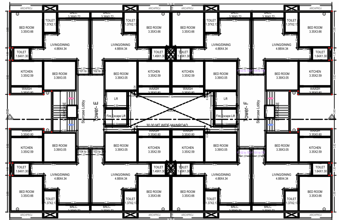
1 ST -7 TH FLOOR PLAN TOWER E & F
