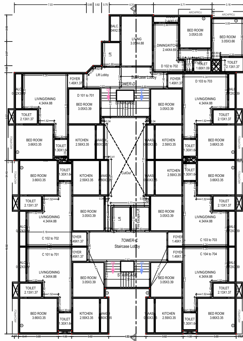
1 ST -7 TH FLOOR PLAN TOWER C & D
