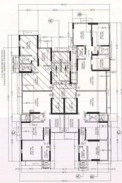
TYPICAL FLOOR PLAN Level to 7th, 9th, To 14th Floor Plan
