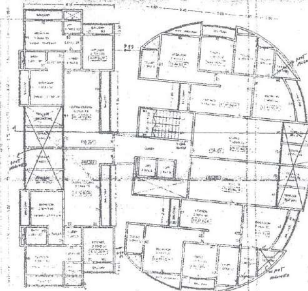
TYPICAL STILT & ST 2ND FLOOR PLAN
