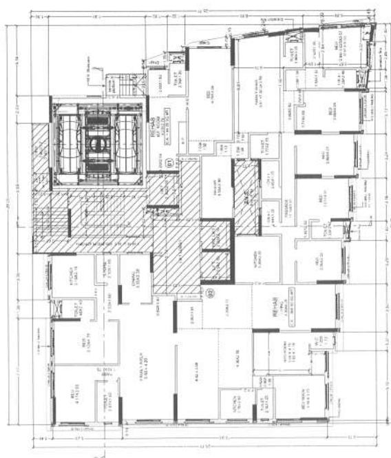
18TH FLOOR PLAN
