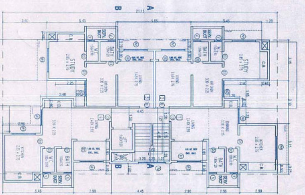
TYPICAL FLOOR PLAN (RESIDENTIAL) SCALE: 1:100
