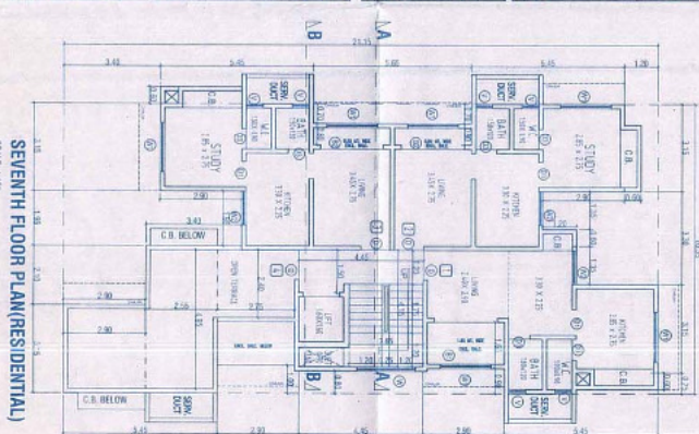
SEVENTH FLOOR PLAN (RESIDENTIAL) SCALE: 1:100
