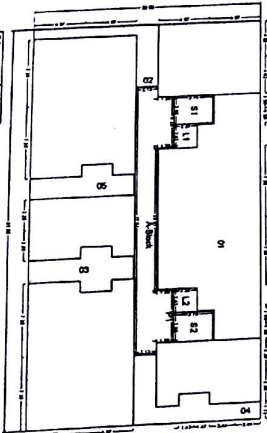
EIGHTH FLOOR PLAN
