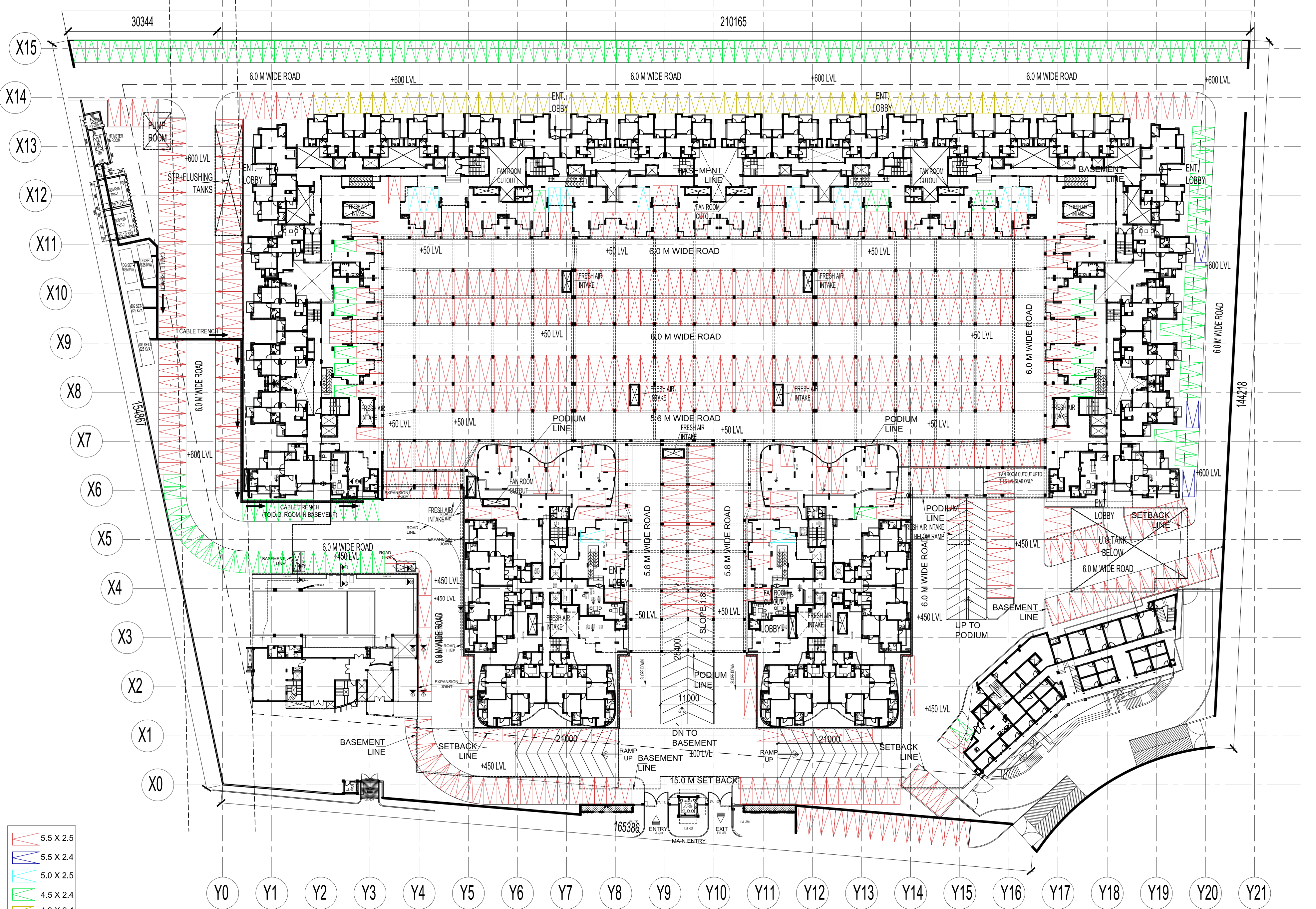
GROUND-SITE PLAN
