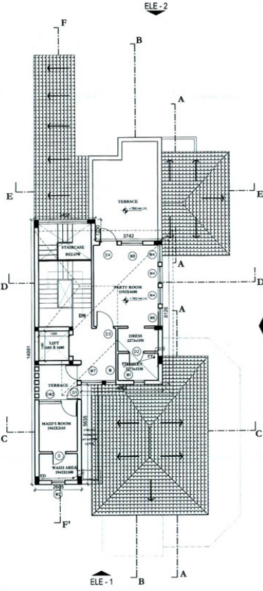
SECOND FLOOR PLAN 1:100
