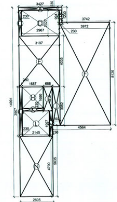
SECOND FLOOR ENVELOPE PLAN 1:100
