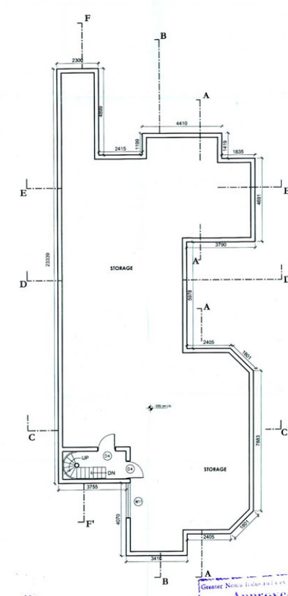
BASEMENT PLAN 1:100
