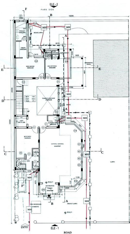
GROUND FLOOR PLAN 1:100
