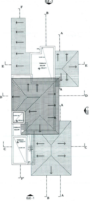
ROOF PLAN 1:100
