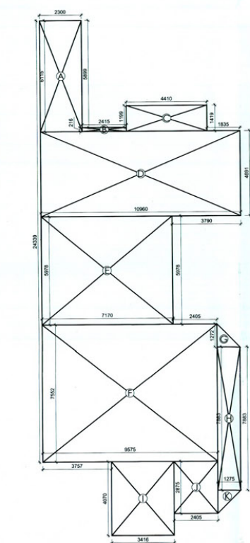
GROUND FLOOR ENVELOPE PLAN 1:100
