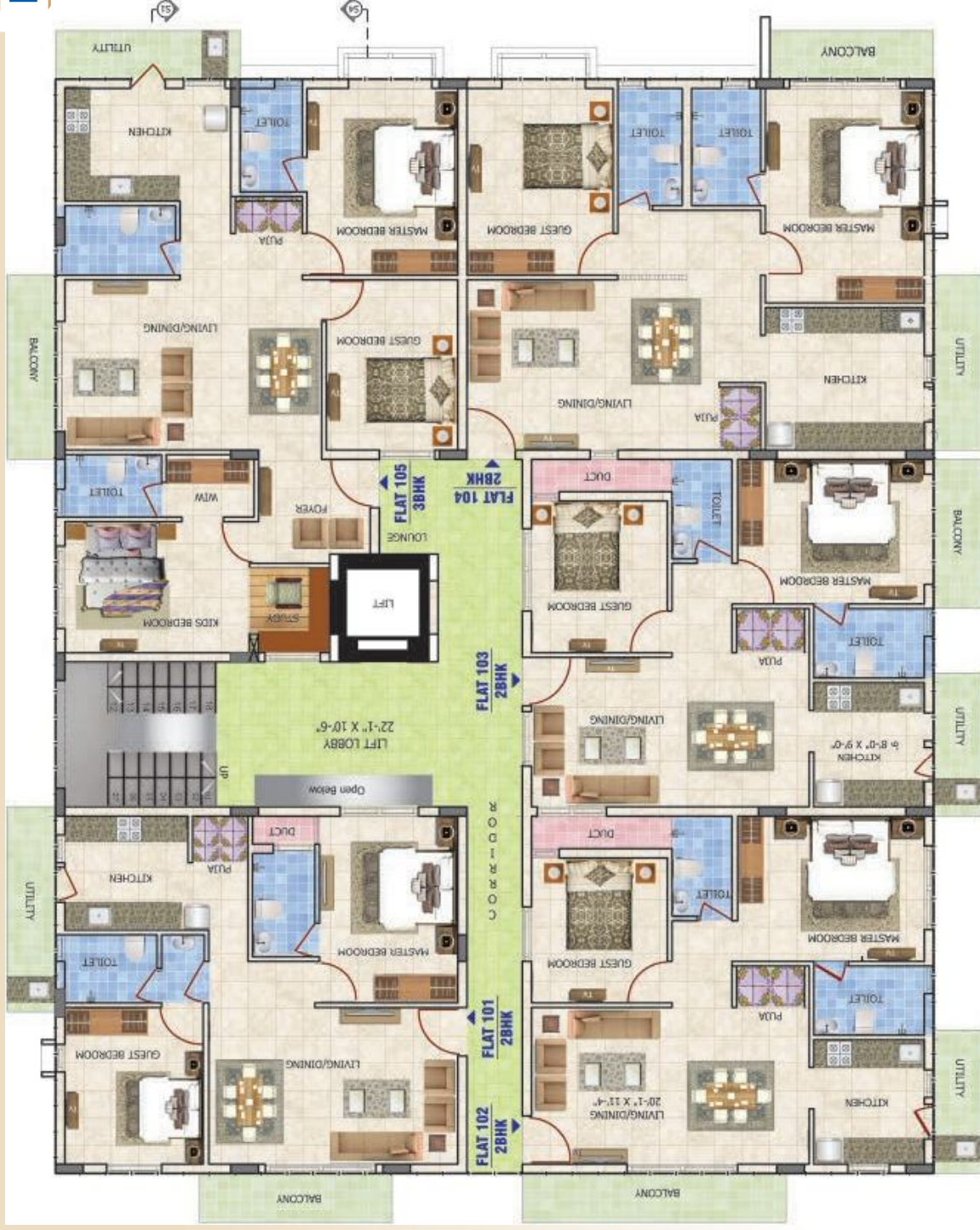
First Floor
