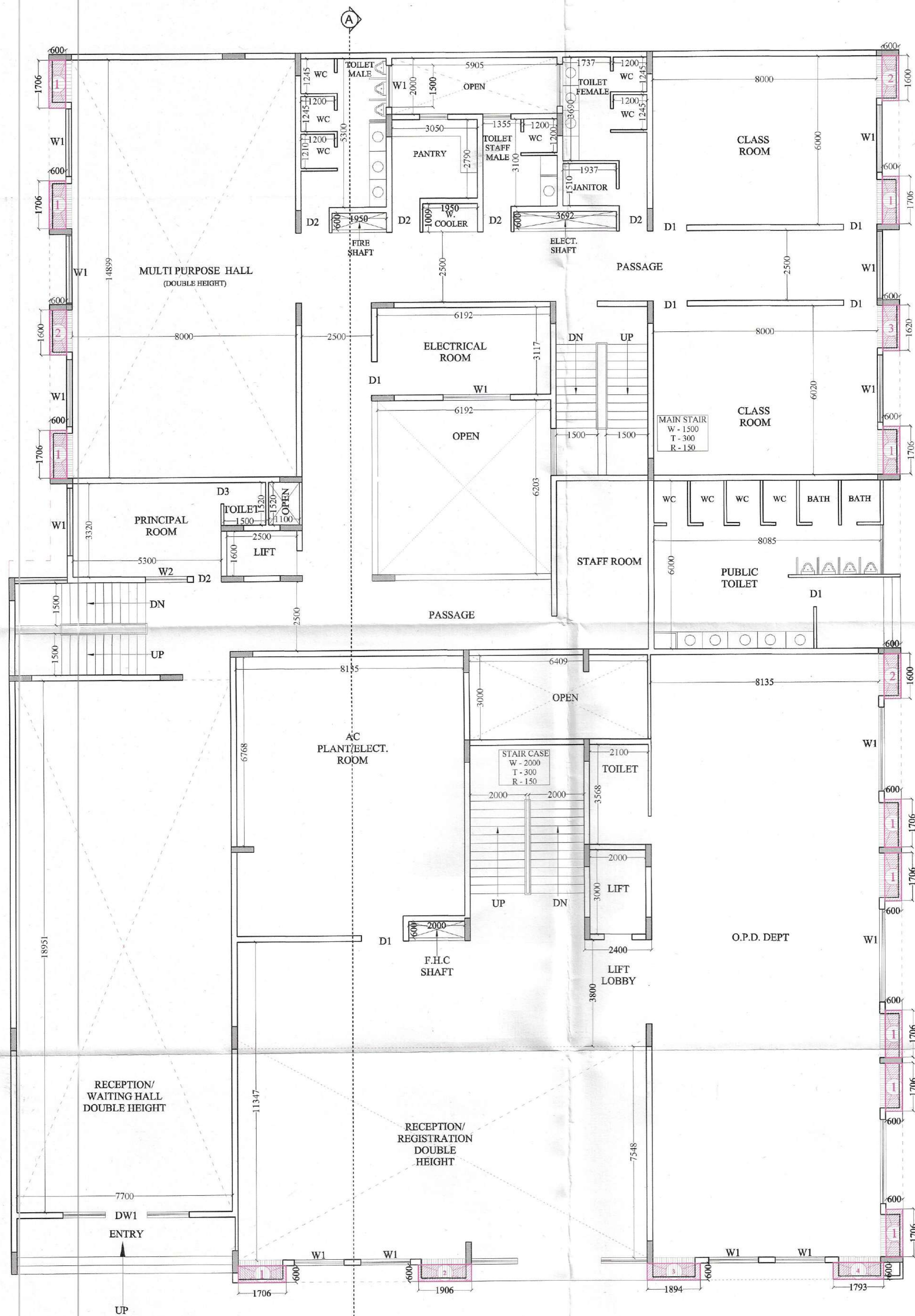
NURSERY SCHOOL GROUND FLOOR PLAN
