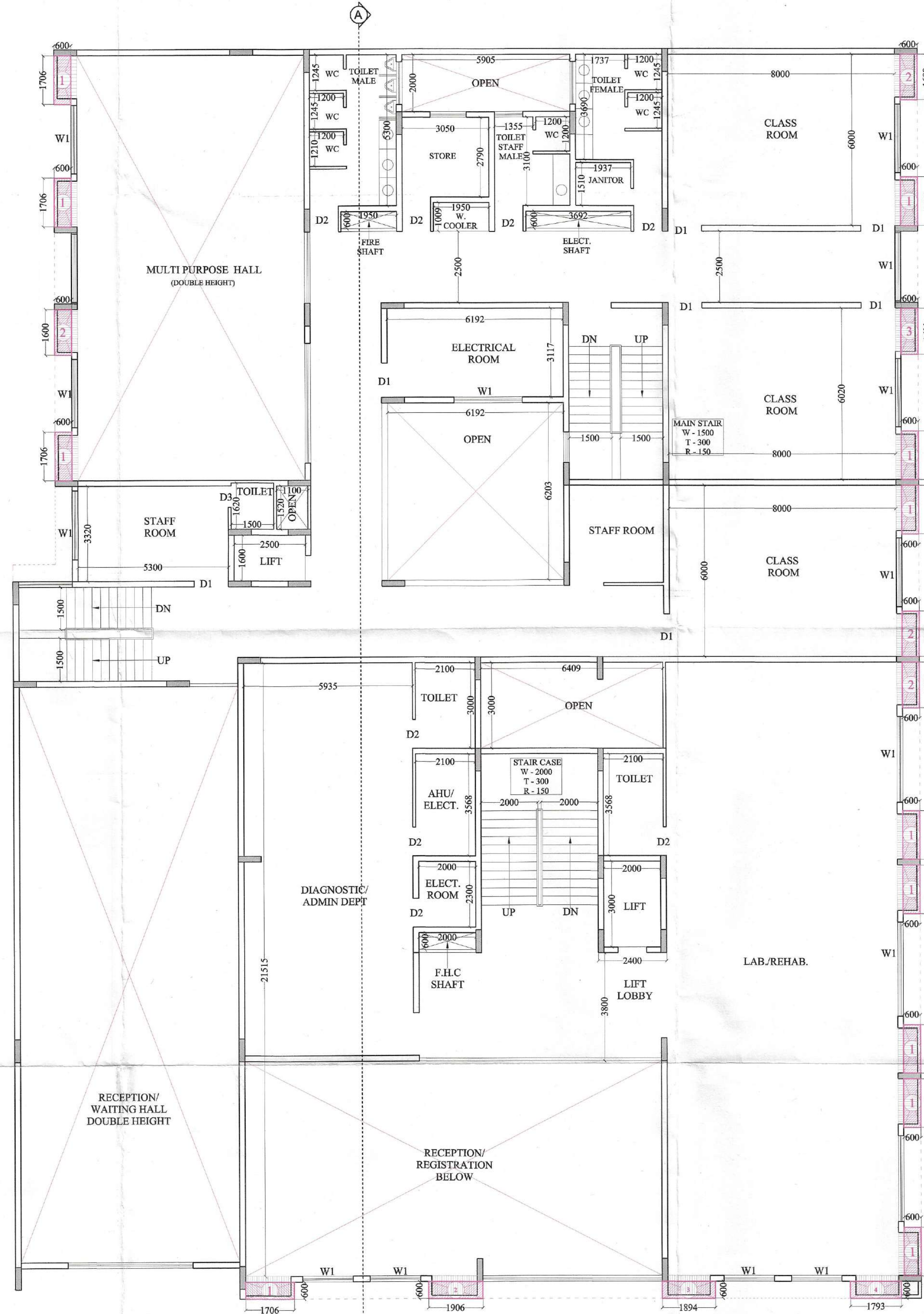
DISPENSARY 1st. FLOOR PLAN
