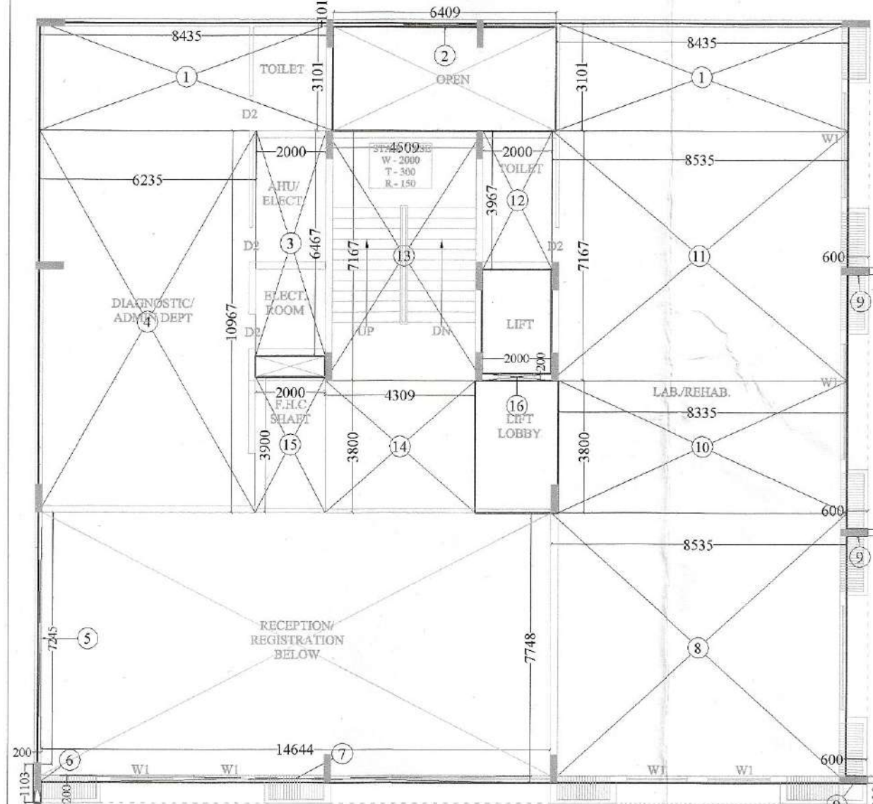
F.A.R. AREA DETAIL OF 1st FLOOR
