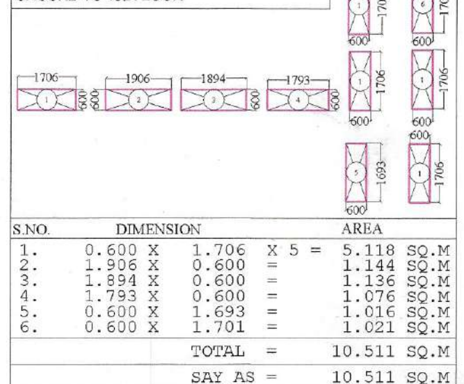
15% FACILITY AREA DETAIL OF CUPBOARD GROUND TO 1st FLOOR
