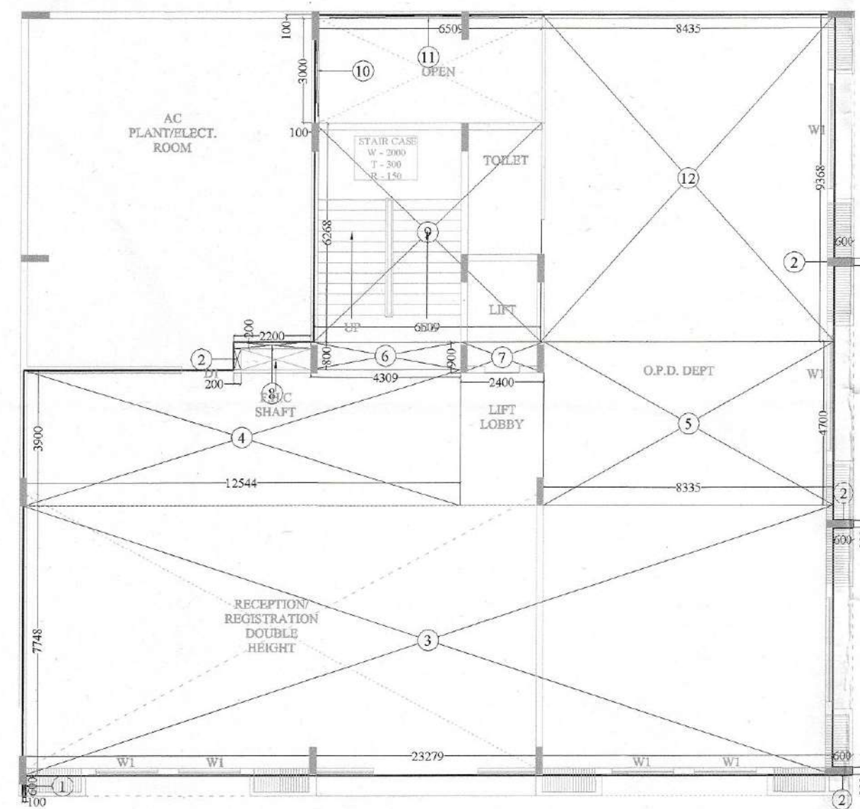
F.A.R. AREA DETAIL OF GROUND FLOOR AREA DETAIL
