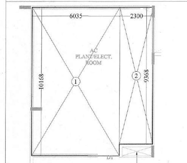
15% FACILITY AREA DETAIL OF ELECTRICAL ROOM GROUND TO 1st FLOOR
