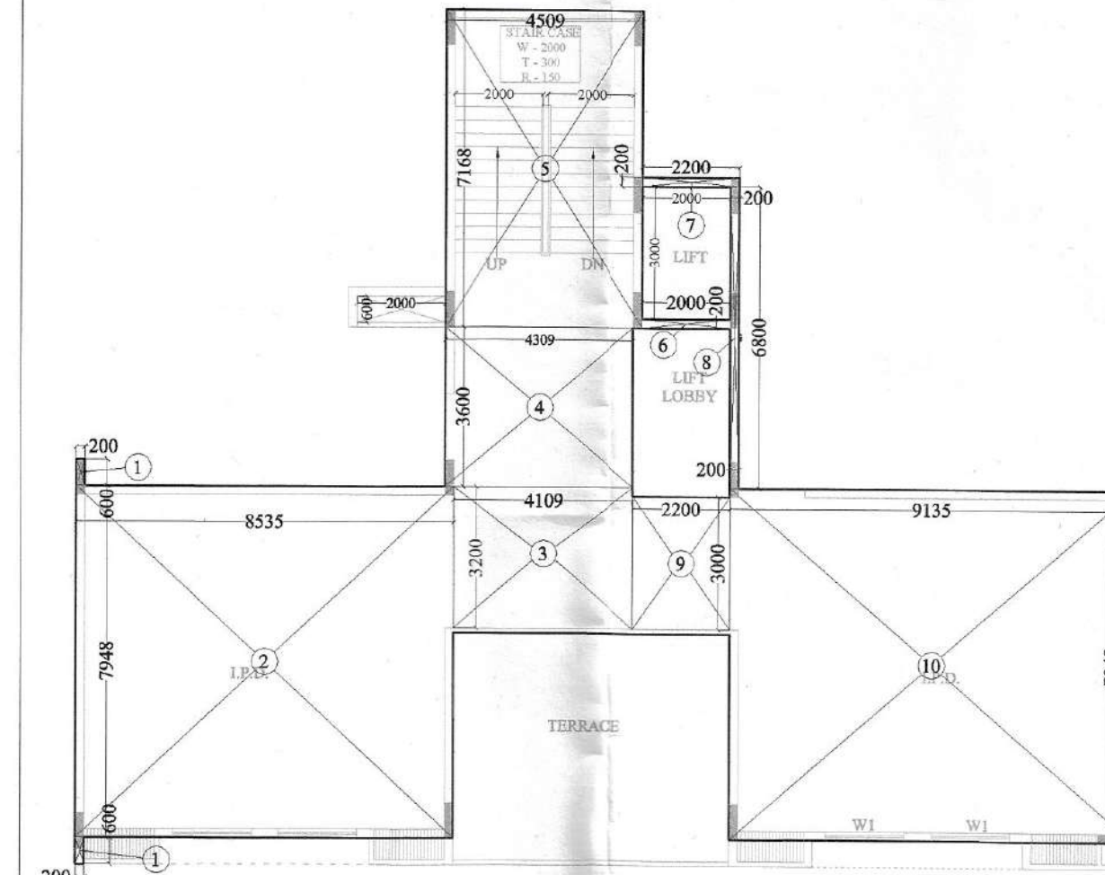
F.A.R. AREA DETAIL OF 2nd FLOOR
