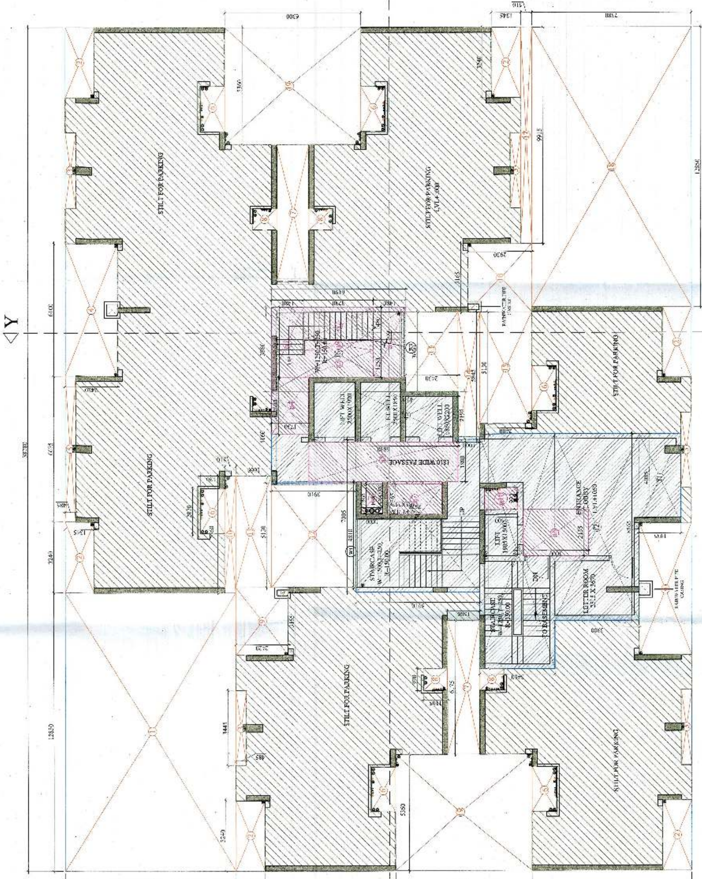
STILT/GROUND LVL. PLAN
