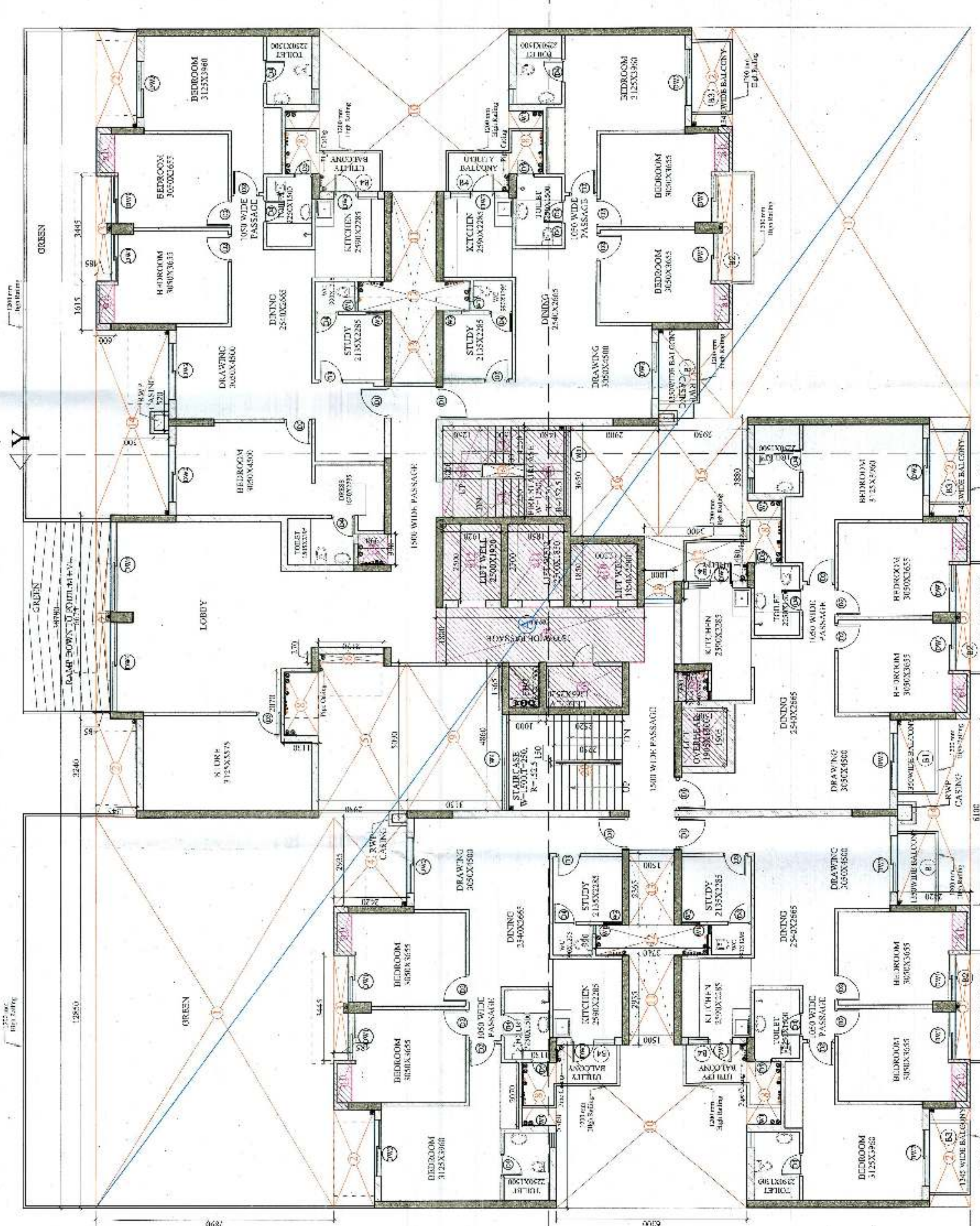
TYPE B - FIRST FLOOR PLAN
