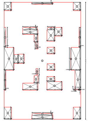
AREA DIAGRAM OF 1ST FLOOR (RESIDENTIAL) SCALE - 1:100
