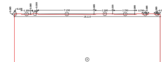
AREA DIAGRAM OF FIRST FLOOR (FITNESS CENTER/SOCIETY OFFICE) SCALE - 1:100
