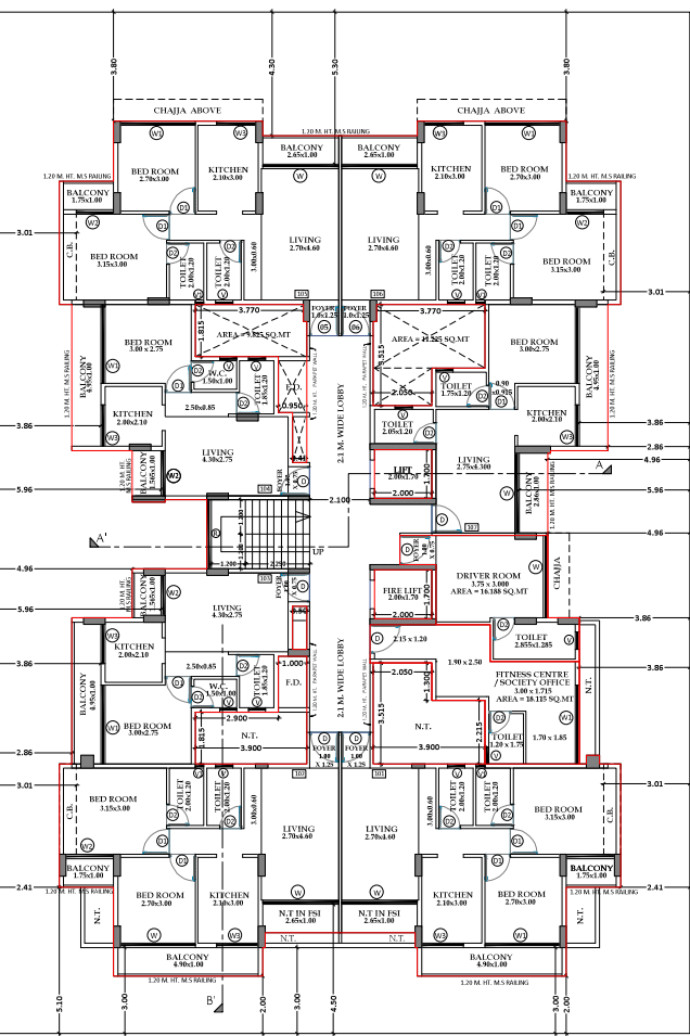
1ST FLOOR PLAN SCALE - 1:100
