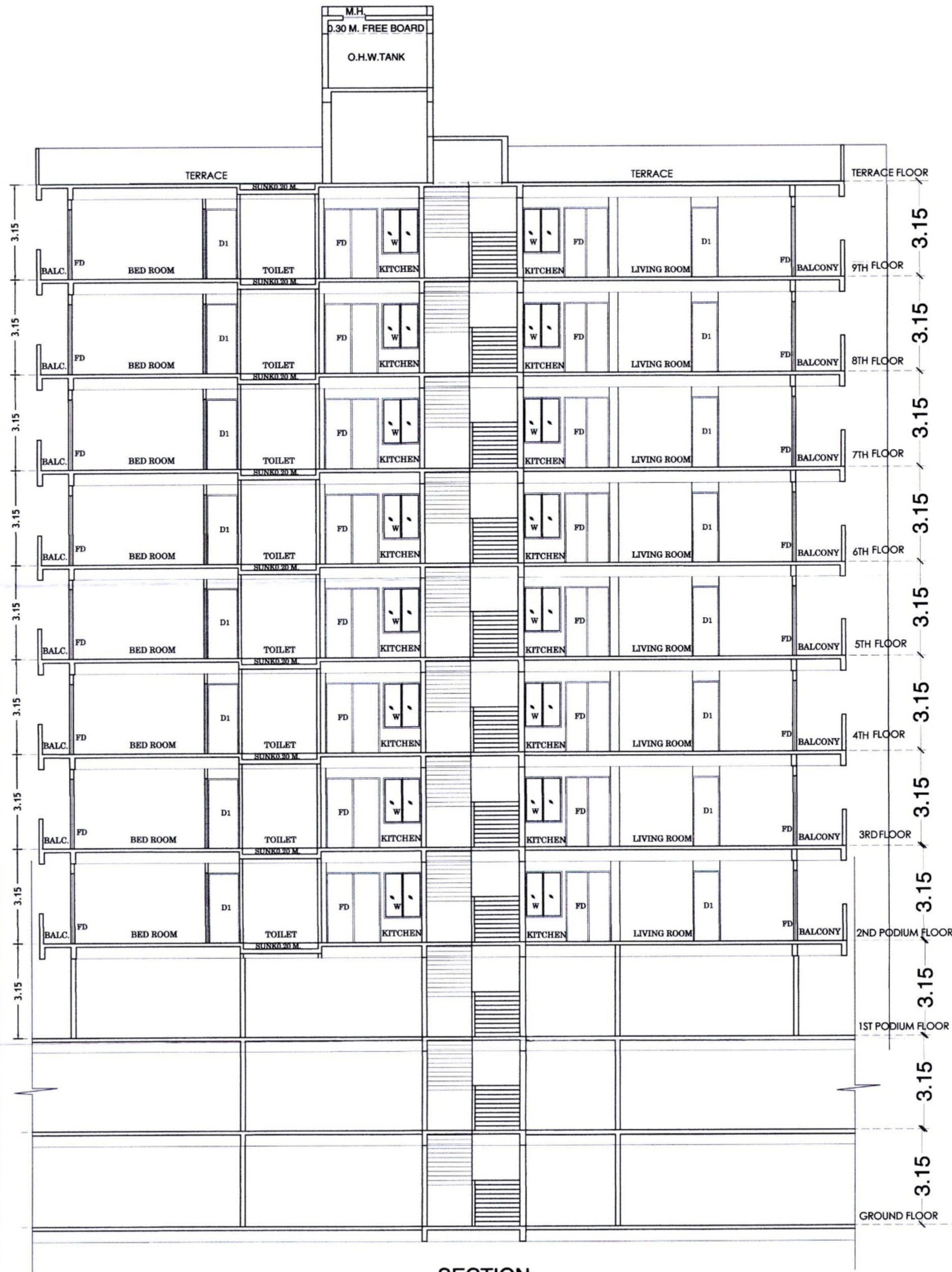
SECTION WING-A'A"
