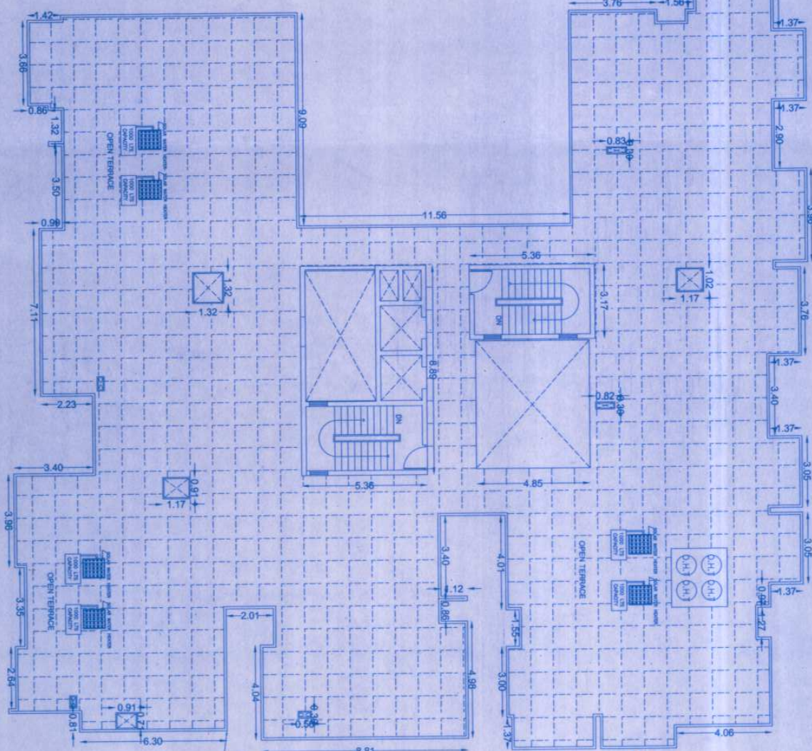
TERRACE FLOOR
