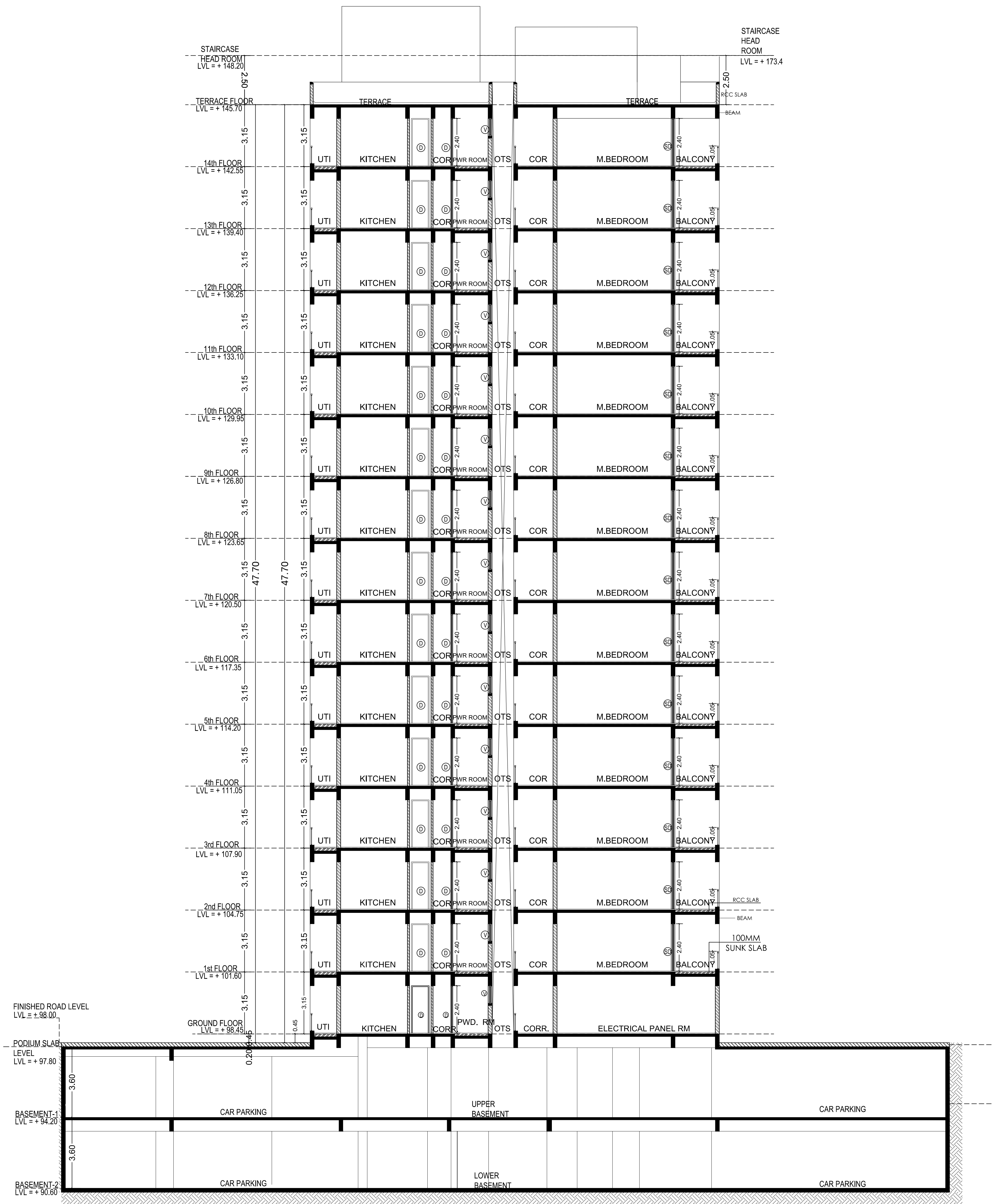
BUILDING SECTION
