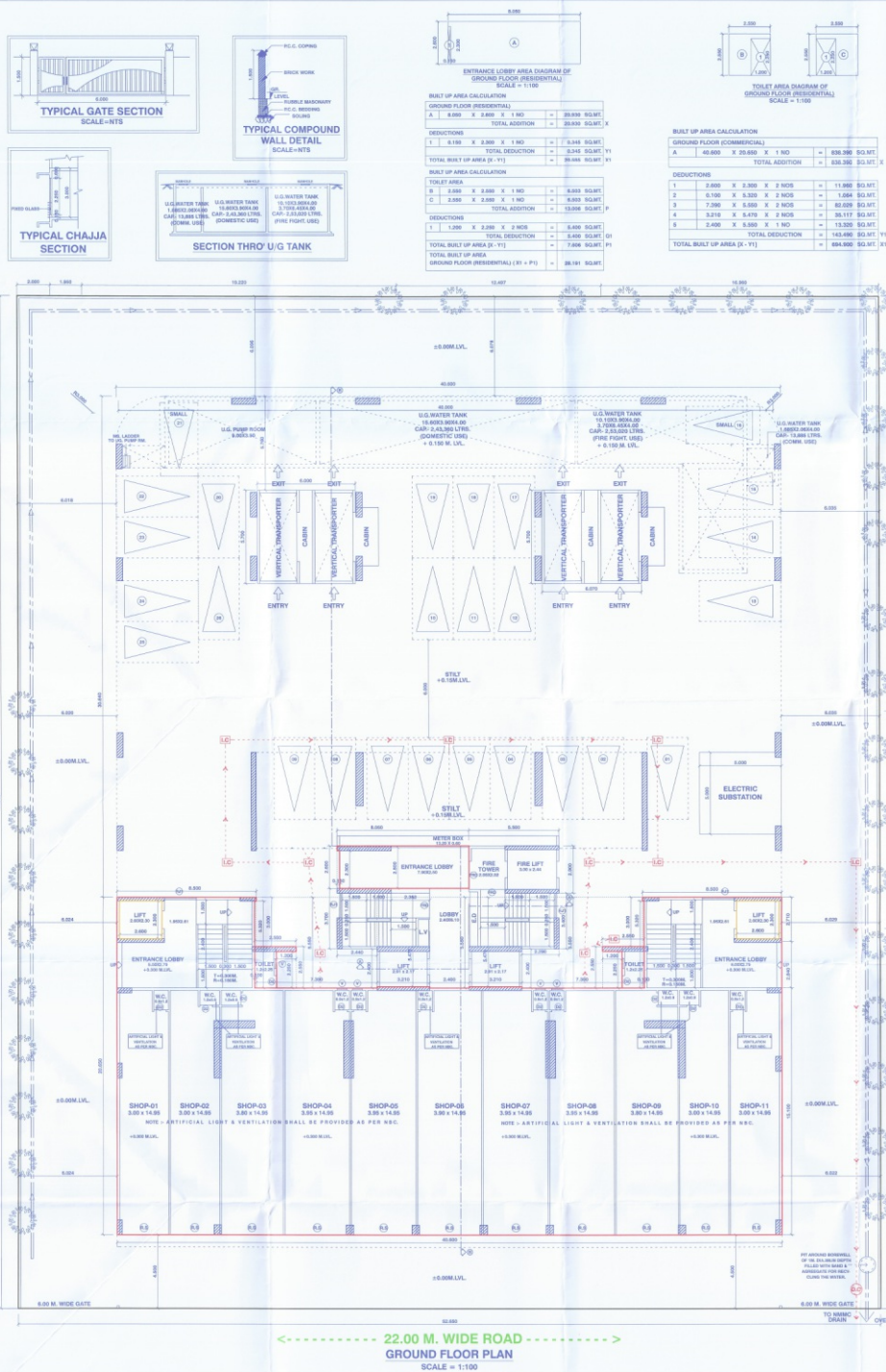
AREA DIAGRAM OF GROUND FLOOR (COMMERCIAL) SCALE = 1:100
