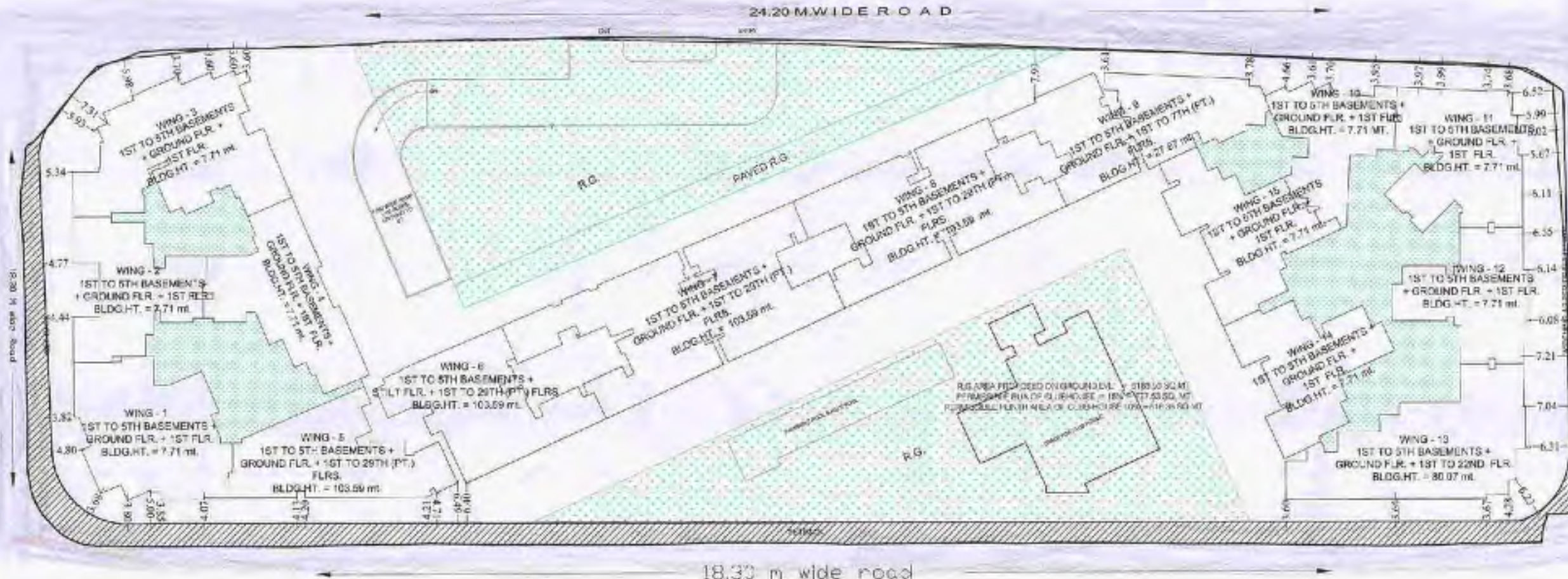
BLOCK PLAN SCALE - 1:500
